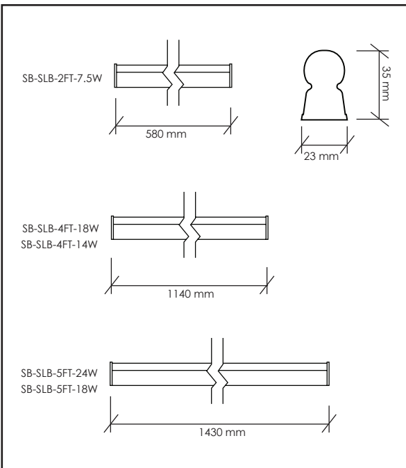
TECHNICAL DRAWING
